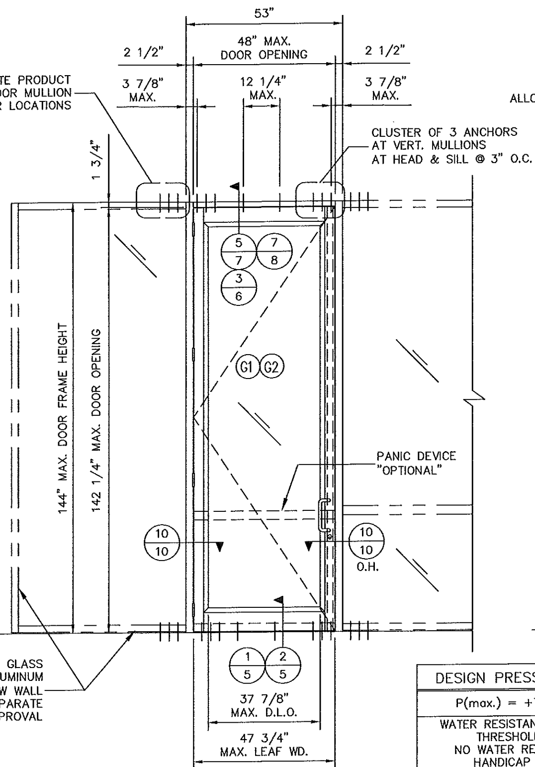
TYPICAL ELEVATION
