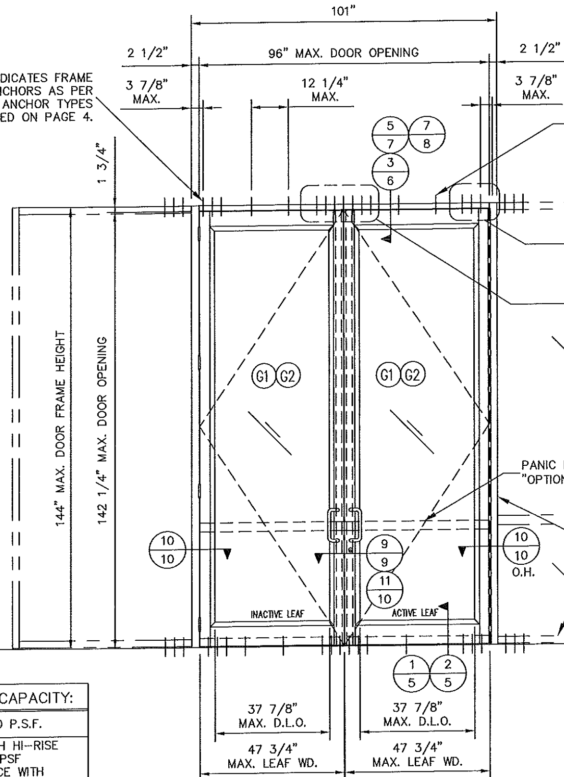
TYPICAL ELEVATION
